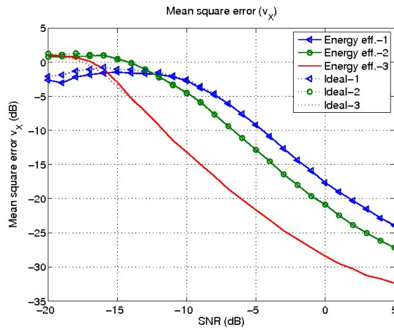
Figure 9: Mean square error of estimated velocity in the x-direction (unit 1 (m/s)^2 ) as function of receiver SNR for all three target scenarios. Here the ideal detector is compared with the energy efficient (that uses data censoring).
