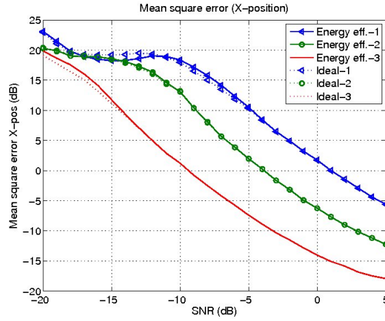
Figure 8: Mean square error of estimated position in the x-direction (unit 1 m^2 ) as function of receiver SNR for all three target scenarios. Here the ideal detector is compared with the energy efficient (that uses data censoring).
