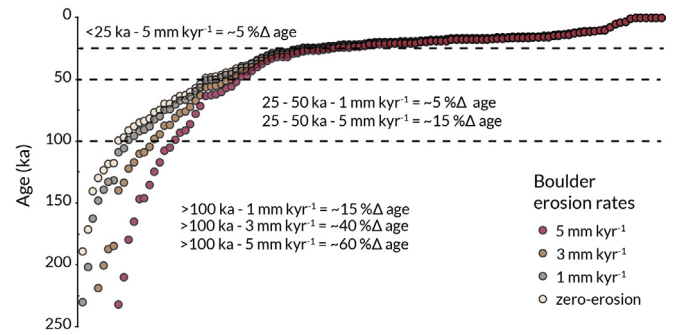
Fig. 9. All 10 Be exposure ages in the Tian Shan related to moraines with at least 3 samples (n = 114; see text for references), sorted oldest to youngest, and the effect of boulder erosion rates of 1, 3, and 5 mm kyr -1 , using the nuclide specific LSD scaling and the updated global reference production rate of Heyman et al. (2016). (For interpretation of colour in this figure, the reader is referred to the web version of this article.)
