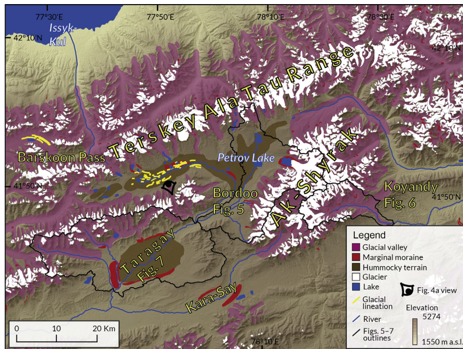
Fig. 3. Glacial geomorphology of the Ak-Shytrak area in the central Kyrgyz Tian Shan (Stroeven et al., 2013). Location of map is shown in Fig. 2. Also shown is Fig. 4a view and Fig. 5–7 outlines. (For the figure in colour, the reader is referred to the web version of this article.)
