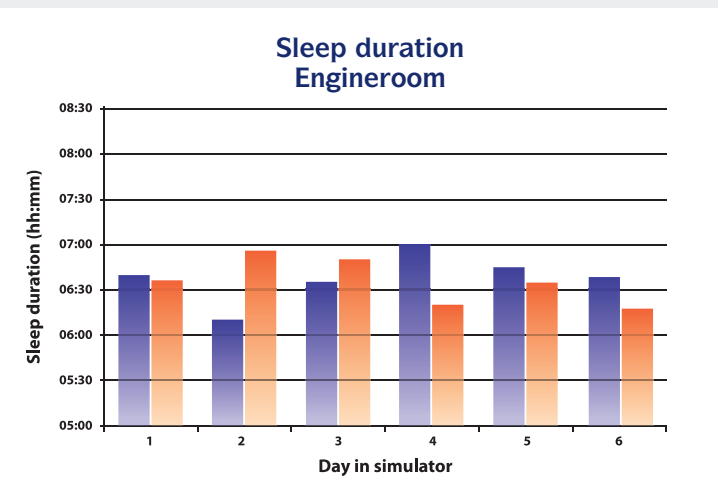
Fig.8 Sleep duration per 24-hour period during the experimental week for Warsash participants working the 6-on/6-off system engineerroom simulators. The team working 0000 to 0600 and 1200 to 1800 is indicated in blue, the team working 0600 to 1200 and 1800 to 0000 in orange
