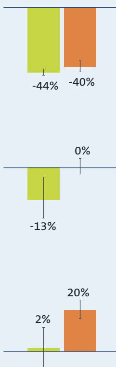
Primary production
